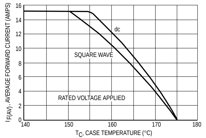
Figure 3. Current Derating, Case (Per Leg)
